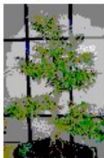
Dithering Floyd-Steinberga
