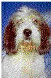
Dithering Floyd-Steinberga
